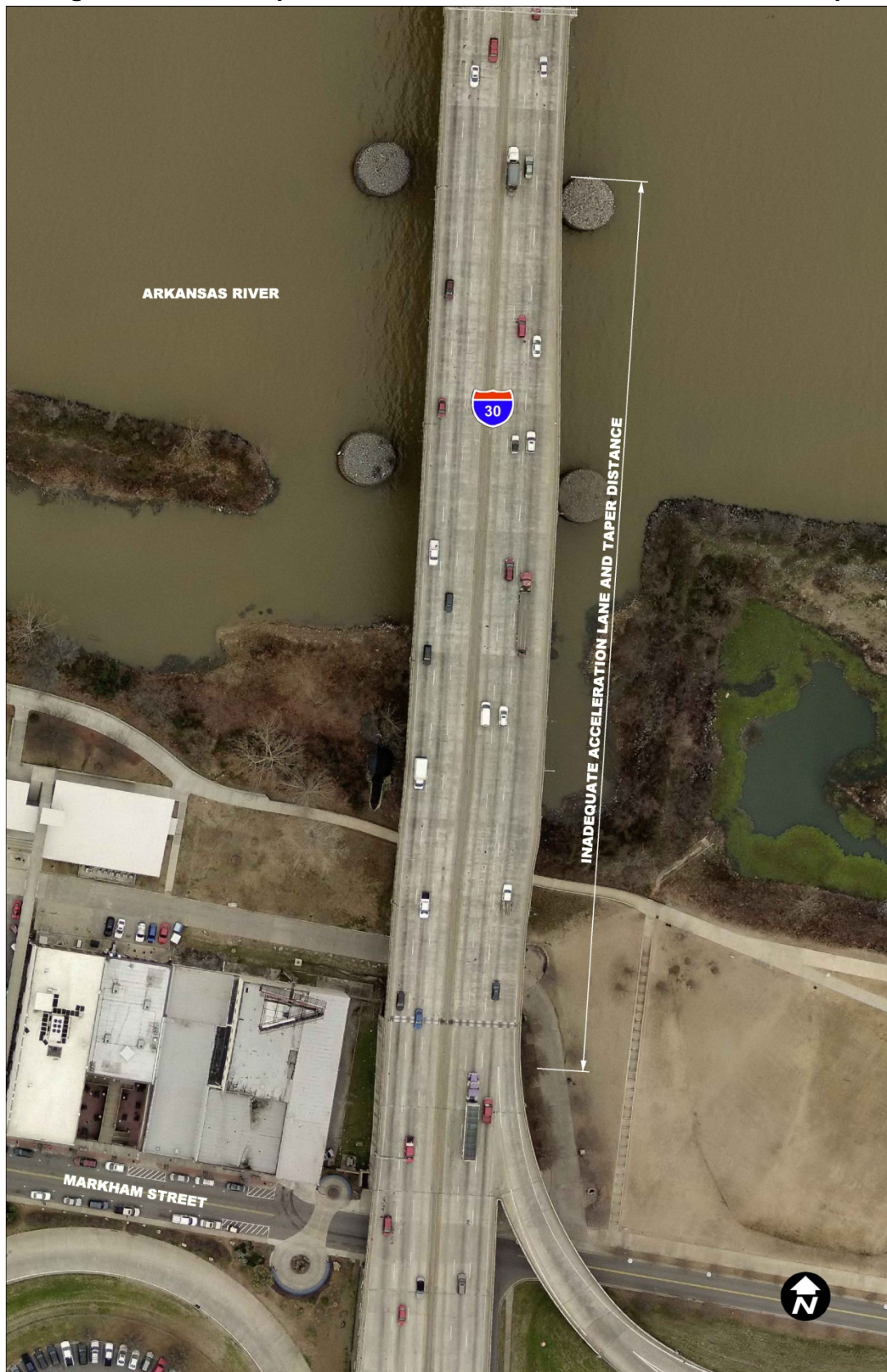
Figure C-5d. Inadequate Acceleration Distance at I-30 Entrance Ramp
